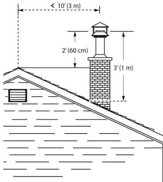
Figure 17 – Min. Chimney Height 1
