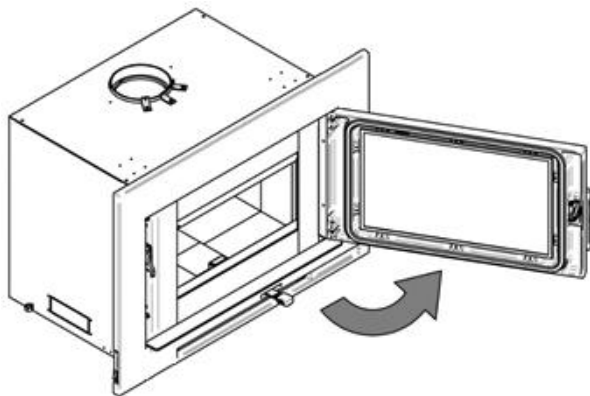
Figure 25 – Open Door
