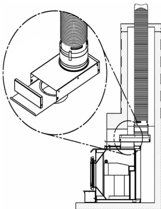
Figure 16 – Offset Adaptor
