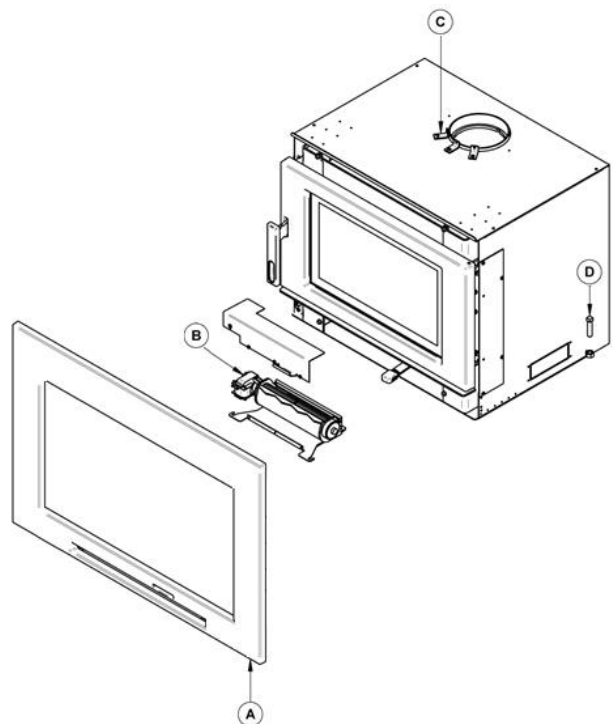
Figure 39 – Insert Removal
